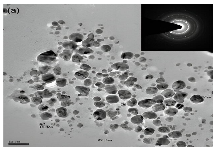
Fig 2. Transmission electron microscopy image of spherical silver nanoparticles in high resolution, measuring 8:20 nm in size "scale bar equal to 50 nm" with an image displaying the selected area electron diffraction (SAED) pattern (Balakumaran et al. 2015).
